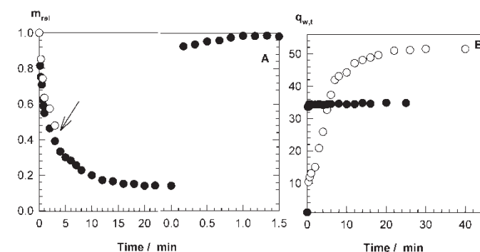
Fig. 5. (A) The relative weight swelling ratio m_{\text{rel}} of PAMPS hydrogels obtained at T_{\text{prep}} = -2^{\circ}\text{C} shown as a function of the time of deswelling in acetone and re-swelling in water. Filled and open circles represent m_{\text{rel}} data of I-and N-gels, respectively. N-gel breaks down during deswelling as indicated by the arrow; (B) The weight swelling ratio q_{w,t} (mass of gel at time t /mass of dry network) of I-gel (filled symbols) and N-gel (open symbols) plotted against the deswelling and swelling times in acetone and water, respectively. T_{\text{prep}} = -2^{\circ}\text{C} . X = 1/6 .
